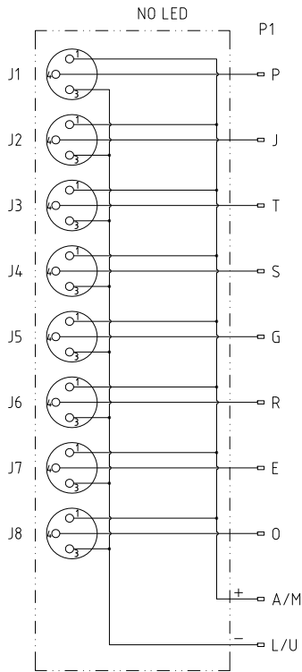
WIRING DIAGRAM
